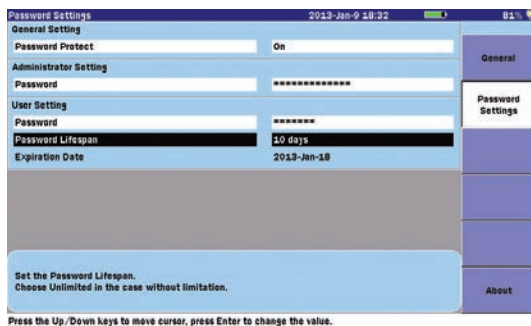
Fig. 10: Password Setting
