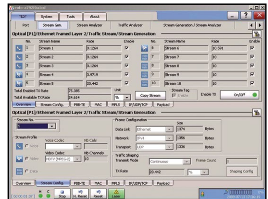
Multistream bandwidth profiles.
