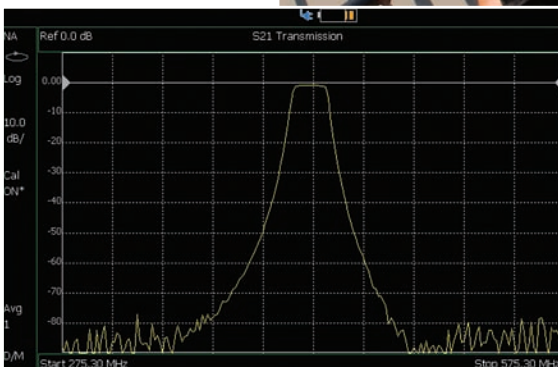
Transmission measurement
