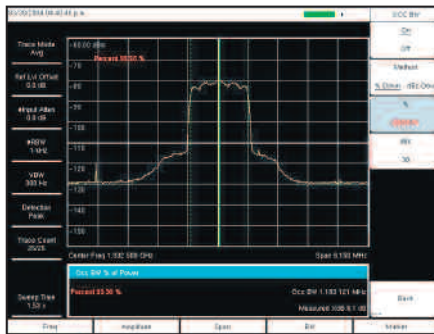
Occupied Bandwidth
