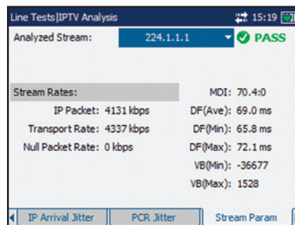
Test results screen showing stream parameters such as MDI.
