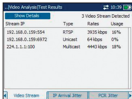
Simultaneous detection of multicast (RTP/UDP), unicast (RTP/UDP) and TCP/RTSP VOD streams.
