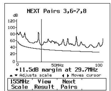
Detailed NEXT results screen shows the measured data as well as the pass/fail limit curve defined by the selected test standard.
