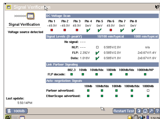
Cable test results, showing PoE detection
