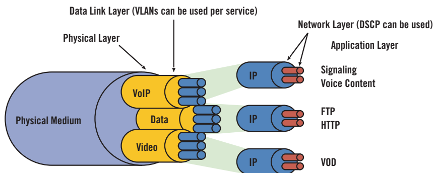
Figure 2. Multiple data streams
