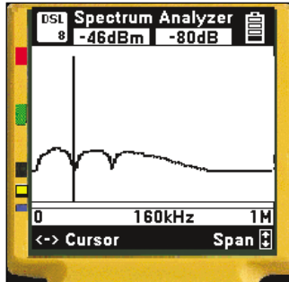
ISDN 2BIQ Cross-talk
