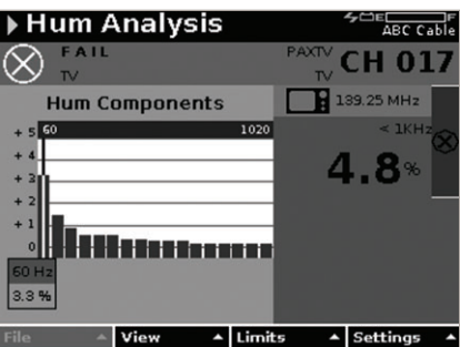
Undesired electrical interference can appear on a video channel as one or two horizontal bars on the TV. A hum measurement reveals if any electrical interference is present on the tested channel.
