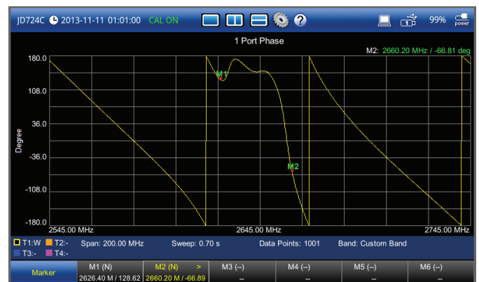
1-Port Phase
