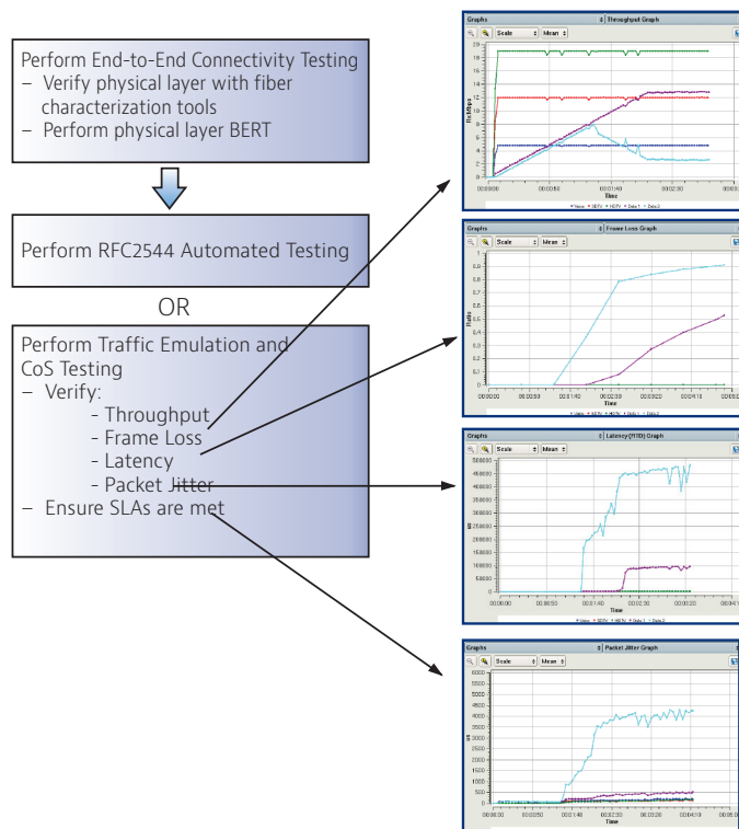
Figure 4. QoS testing
