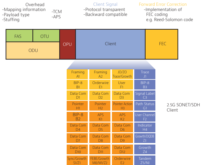
Figure 8. OTN Frame
