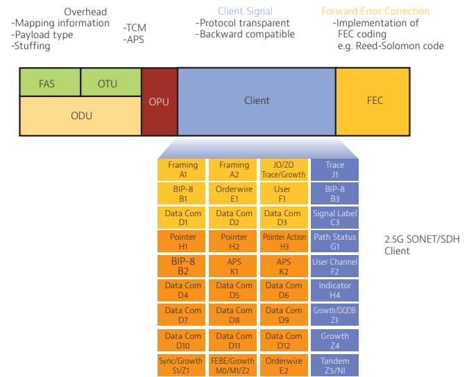
Figure 8. OTN Frame
