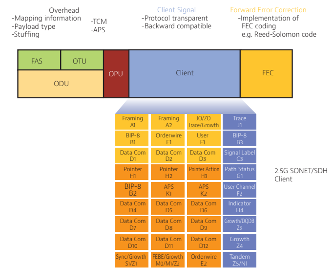
Figure 8. OTN Frame
