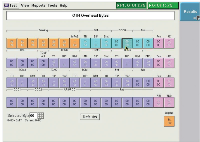
OTN overhead byte manipulation
