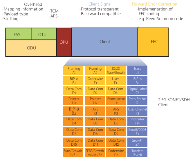
Figure 8. OTN Frame
