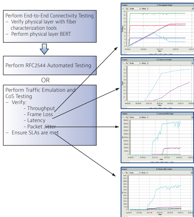
Figure 4. QoS testing
