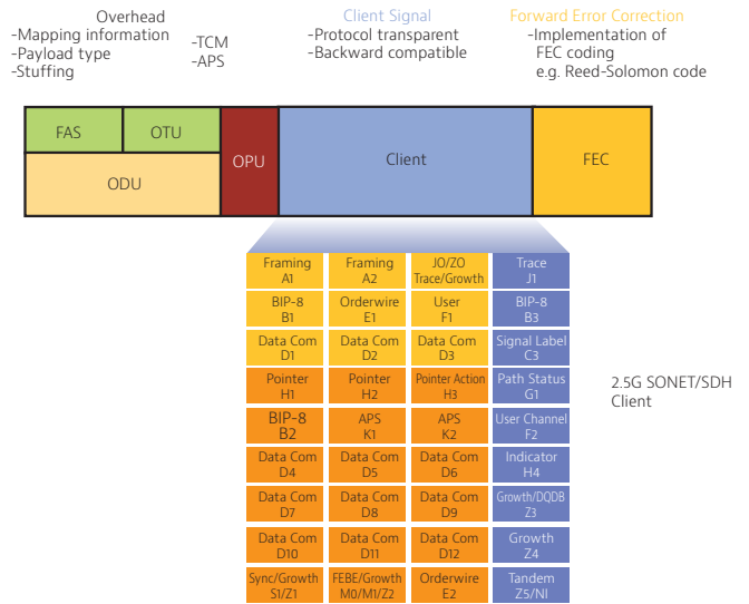
Figure 8. OTN Frame
