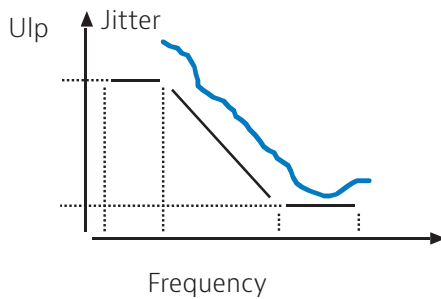
Figure 10 Jitter mask
