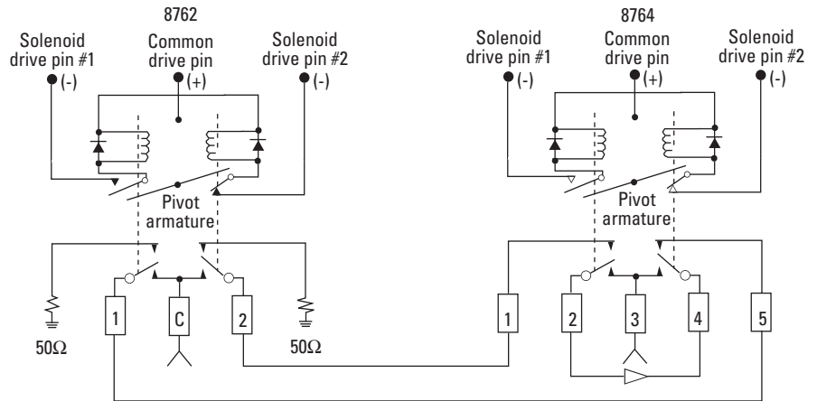
Figure 6. Signal reversal
