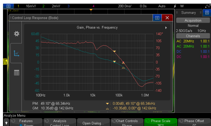
Figure 30b. New control loop response analysis (bode plot) shows the gain/phase plot over frequency sweep.
