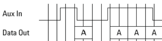
Figure 16: Output blanking
