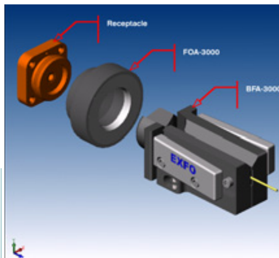
BFA-3000, FOA-3000 and receptacle assembly.
