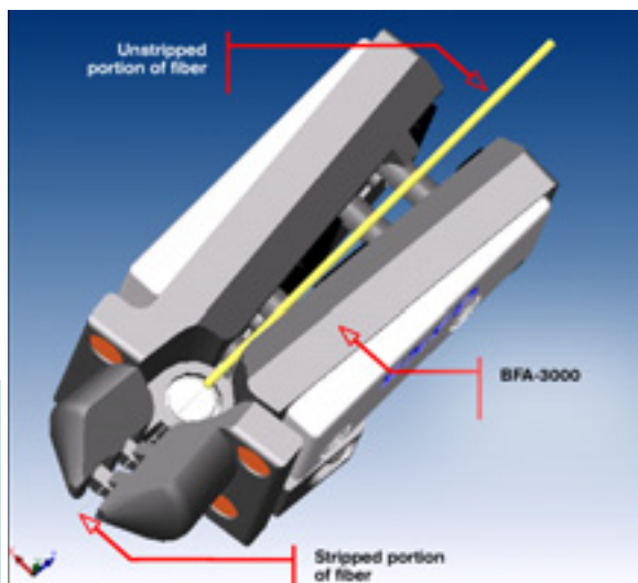
BFA-3000 in open position. Fiber is in place. Yellow portion of fiber is unstripped.
