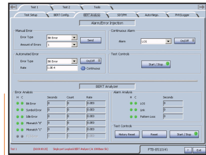
BERT analysis screen
