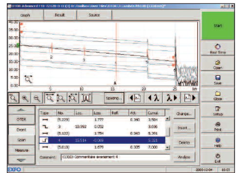
Multiple-trace comparison on the FTB-500.
