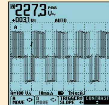
Connect-and-View captures even the most complex motor drive signals.
