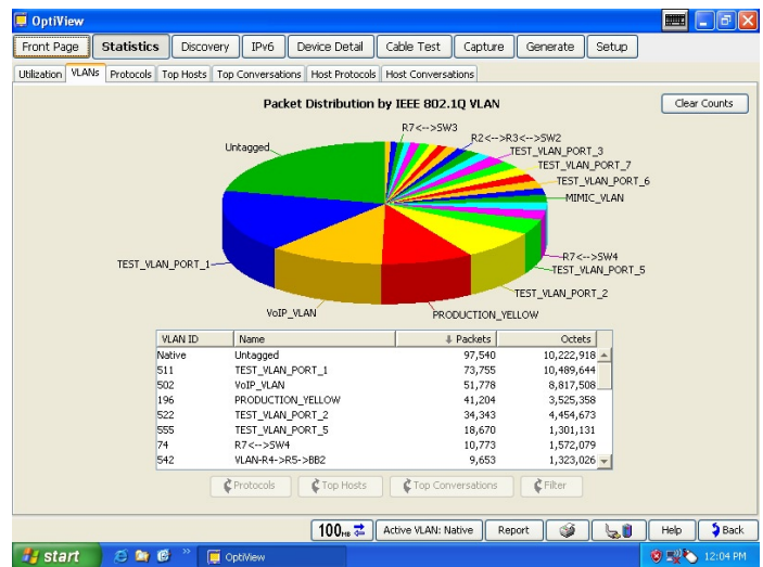
VLAN statistics
