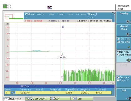
FTTx OTDR testing
