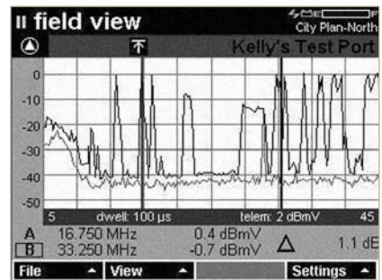
The optional Field View capability greatly improves the success rate and efficiency in chasing down ingress on the return path. Field technicians can view the return spectrum as received by the PathTrak Return Path Monitoring System. Both the remote spectrum and the local spectrum view can be compared on the tech's meter.
