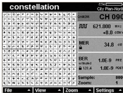
Constellation displays of 64 and 256 QAM carriers are included in the DSAM-3500 and DSAM-3600 models. Demodulation of carriers up to 128,4 deep interleave is supported
