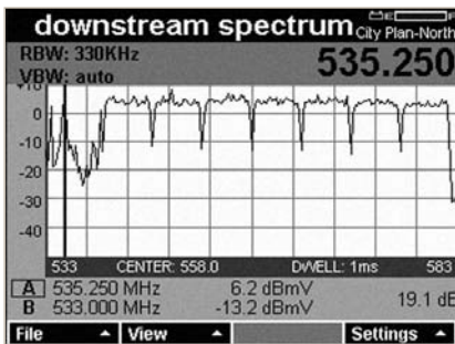
A full downstream spectrum capability is included in the DSAM-3500 and DSAM-3600 models. Carrier characteristics and relationships to adjacent carriers can be quickly seen
