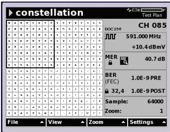
Patterns in the constellation graph display show network impairments. Technicians can figure out the probable cause of the impairment by identifying the pattern.
