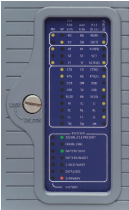
Figure 3. Front panel LEDs monitor signaling and data leads of the circuit under test.
