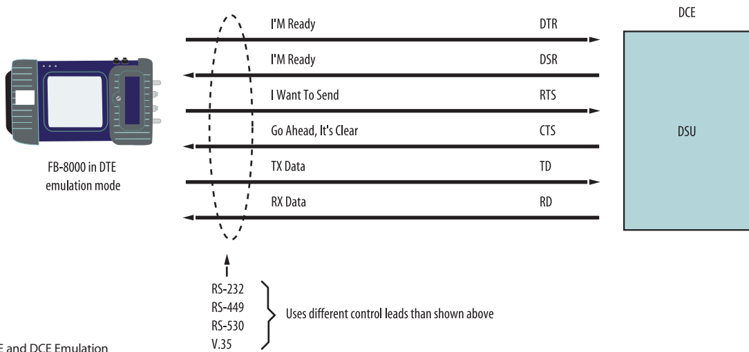
Diagram 2. DTE and DCE Emulation
