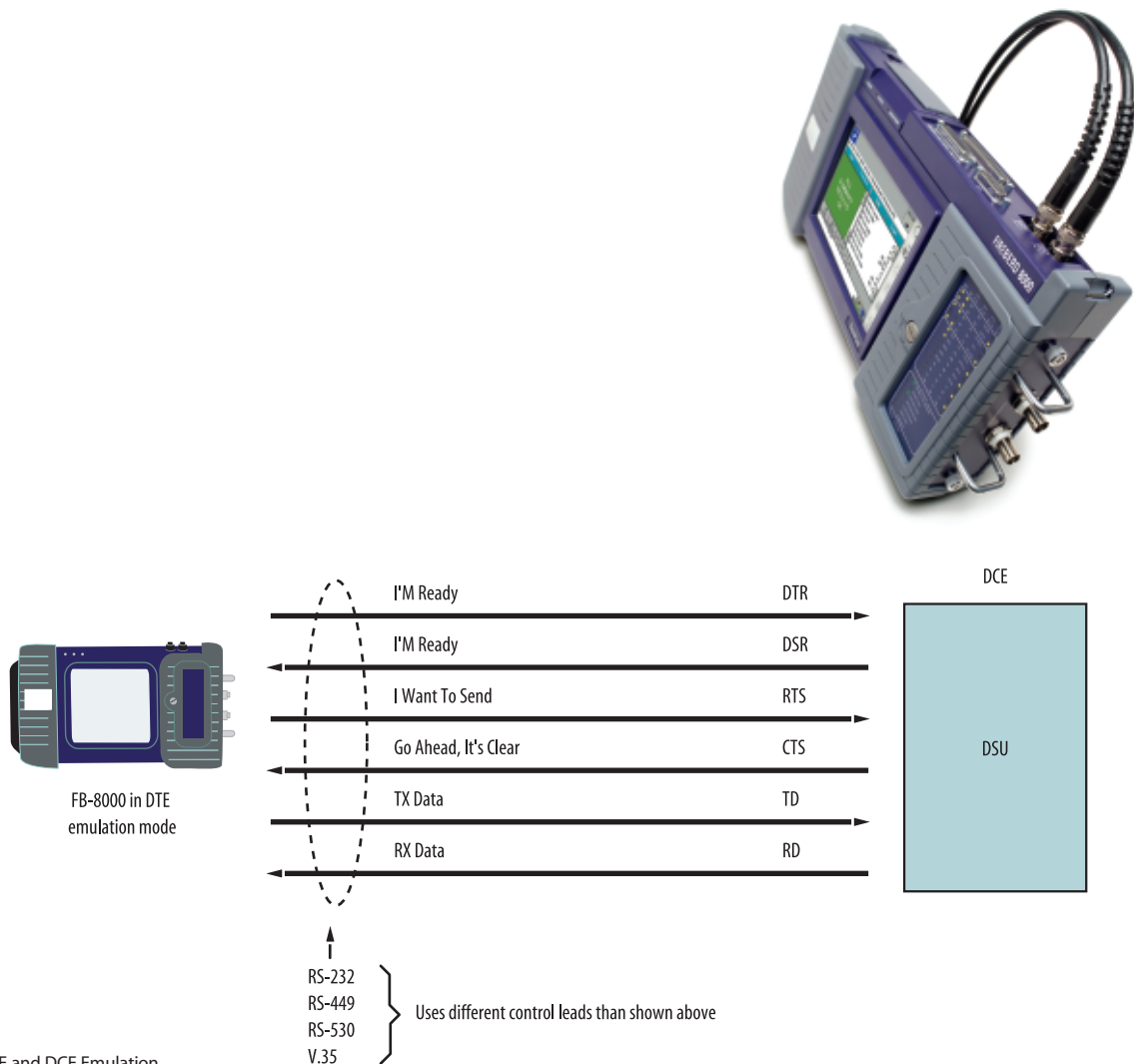
Diagram 2. DTE and DCE Emulation
