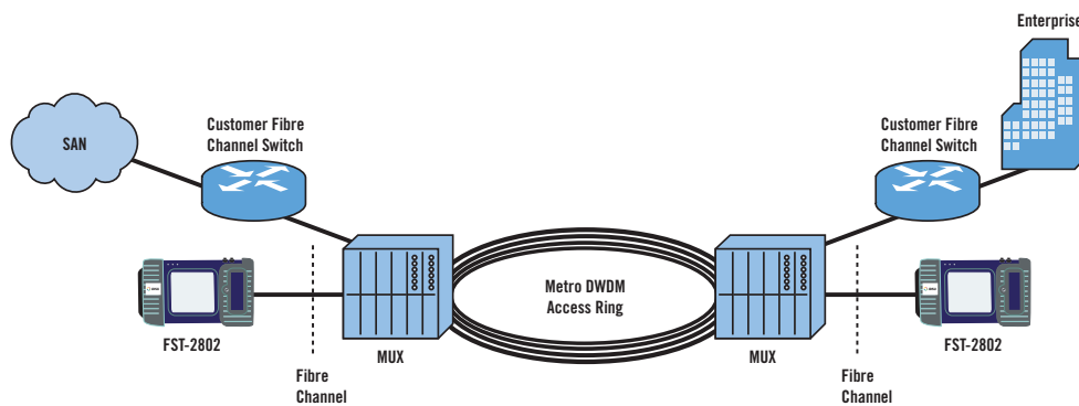
Diagram 3: Fibre Channel testing on a metro DWDM network
