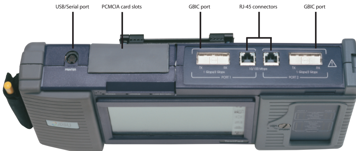
Diagram 4: JDSU FST-2802 dual-port configuration
