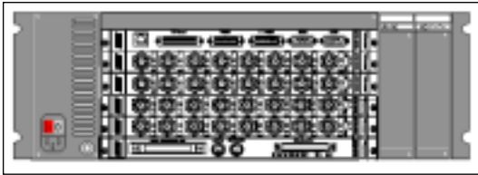
▲ Back view schematic of HCU400 with four RPM1000 modules.
