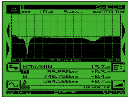
Forward sweep display revealing severe problems at the low frequency end.
