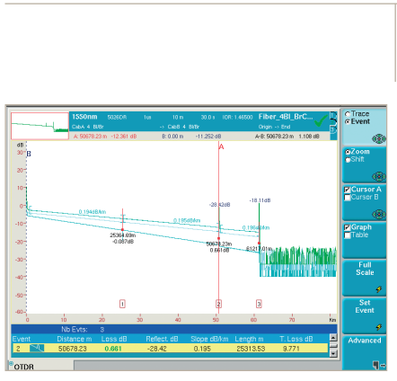
Figure 1 3 wavelength OTDR trace display
