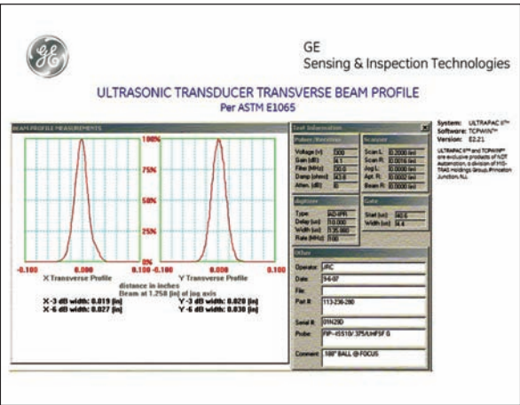
Beam Profile
