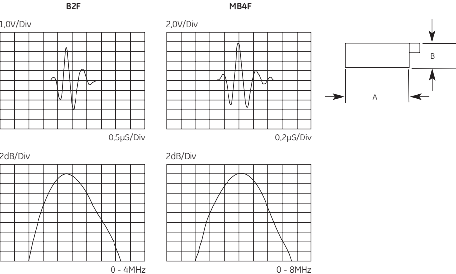
Typical waveform and frequency spectrum
