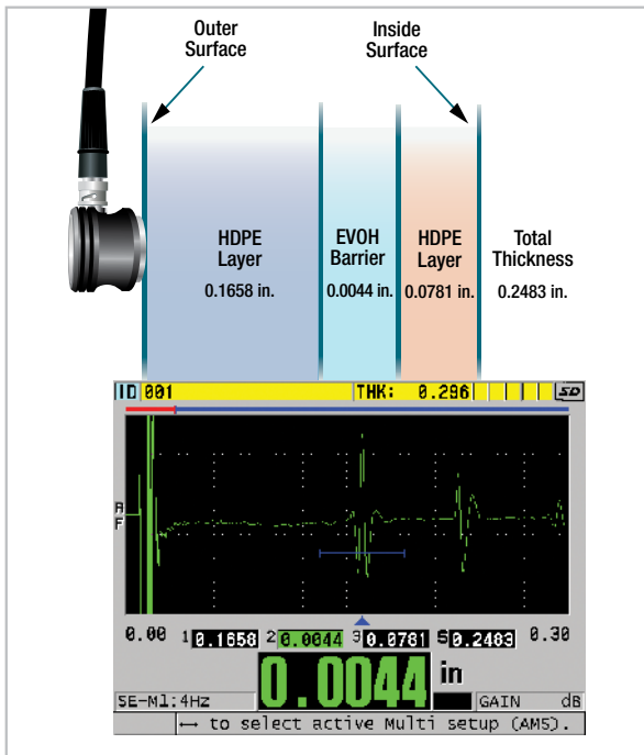
The 38DL PLUS can make accurate measurements of up to four individual layers simultaneously.
