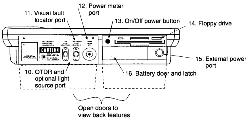
Figure 2-3. Model 7500 back features.
