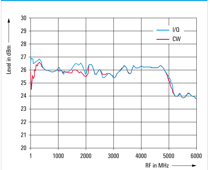
Measured maximum output power versus frequency
