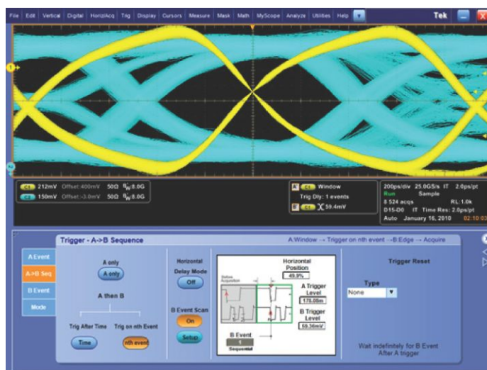
Use B Event Scan trigger on DDR DQS edges used to construct an eye diagram of all bits in a burst.
