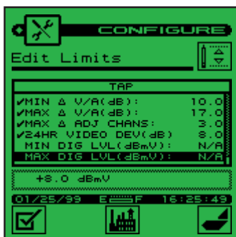
Limit sets for analog channels and a limit set for digital channels.
