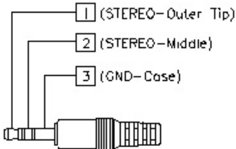
STEREO PLUG DETAIL
