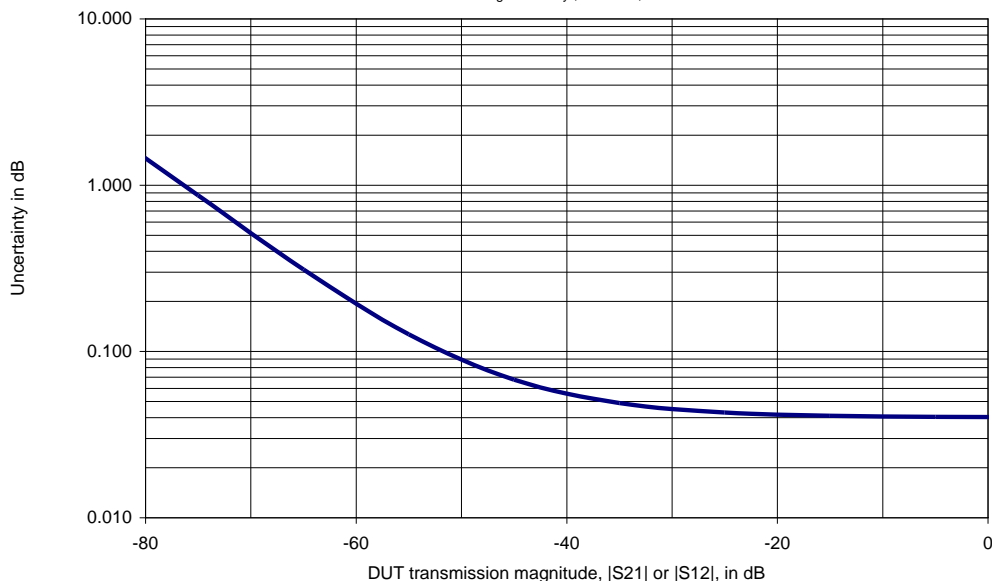
Transmission magnitude uncertainty R&S®FSH4/R&S®FSH8 with the R&S®FSH-K42/R&S®FSH-K45 option.
