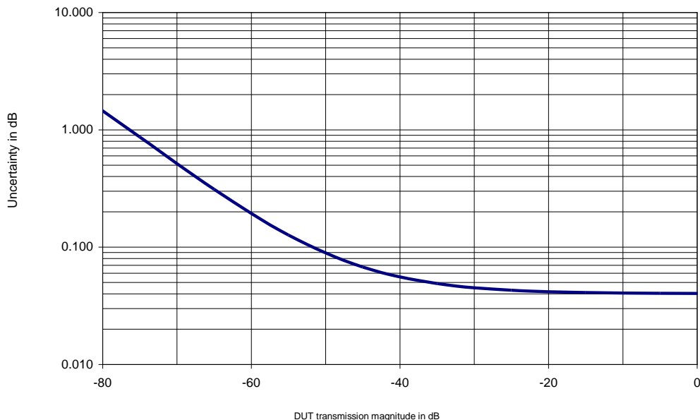
Transmission magnitude uncertainty R&S®FSH13/R&S®FSH20 model .23/30.
