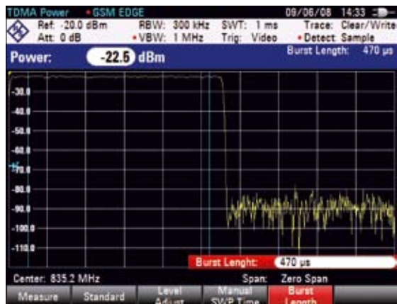
TDMA power measurement
